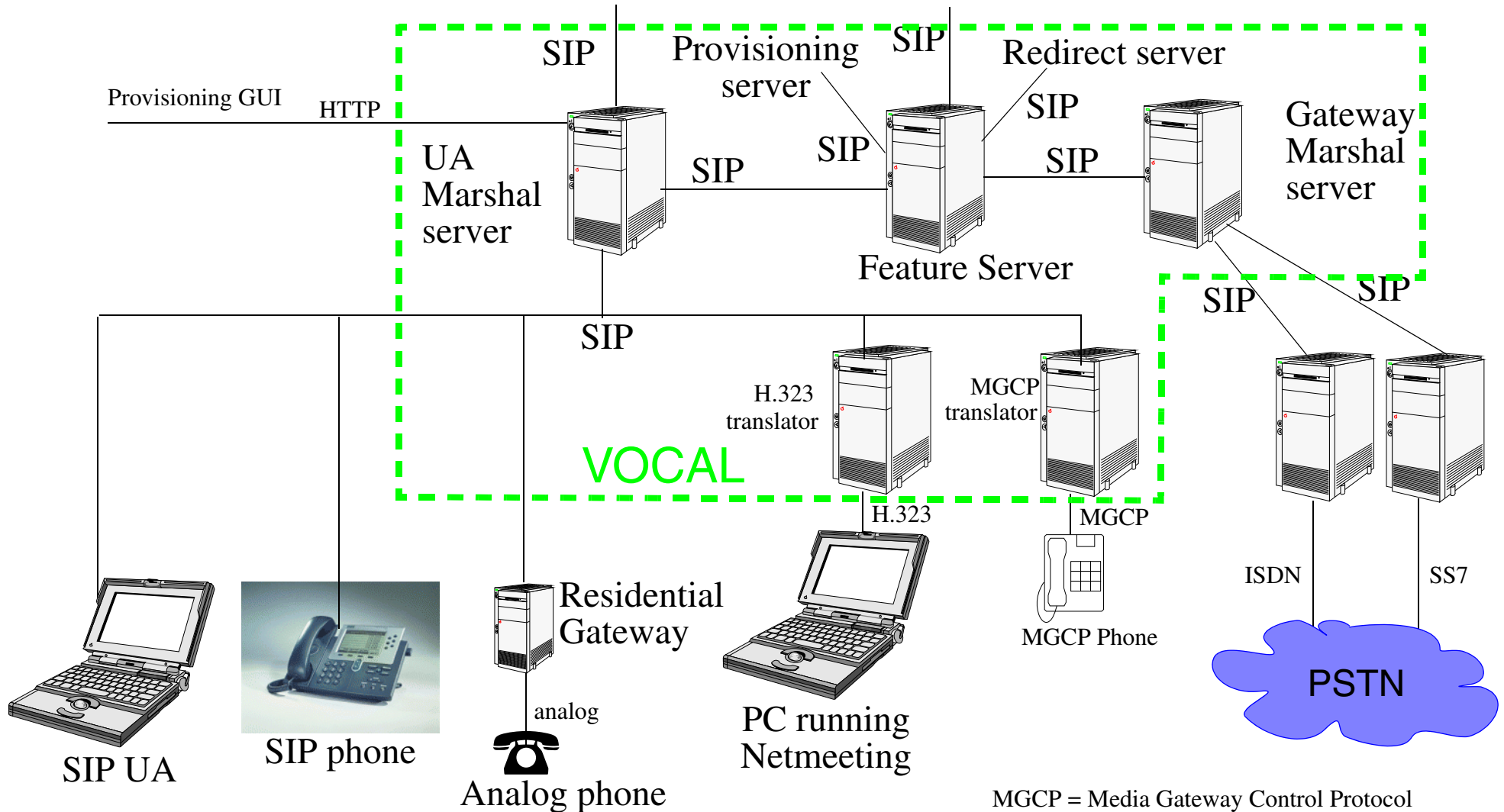
Figure 47: VOCAL: Simplified overview
