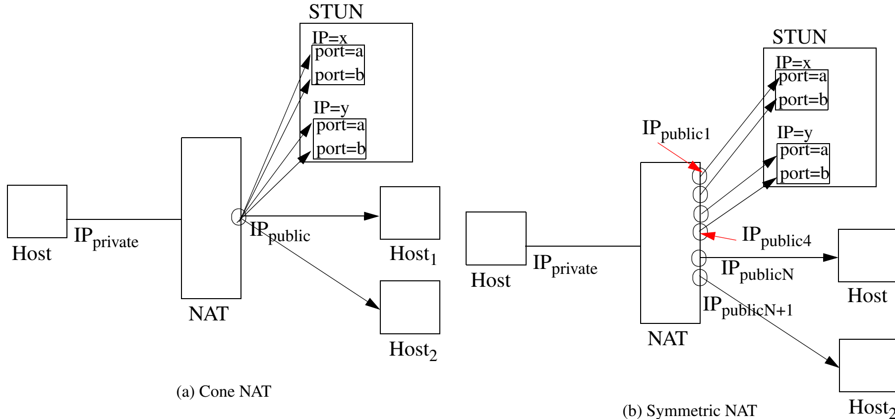
Figure 37: (a) Cone NAT vs. (b) Symmetric NAT - figure inspired by figures 1 and 2 of [246]
