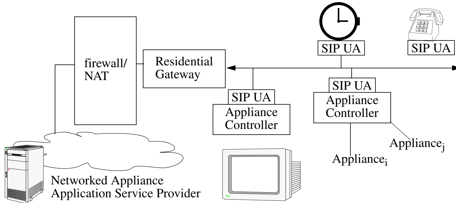
Figure 46: Using SIP for Service Portability (adapted from figure 2 of Moyer, Maples, Tsang, and Ghosh)
