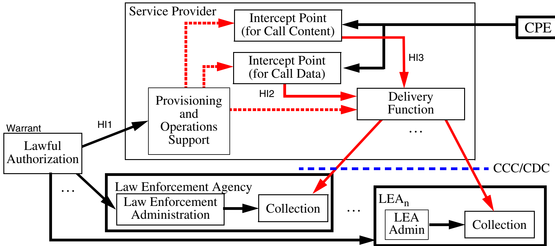
Figure 18: Interfaces in RED should be standard to allow interoperability; HI_n = \text{Handover Interface}_n
