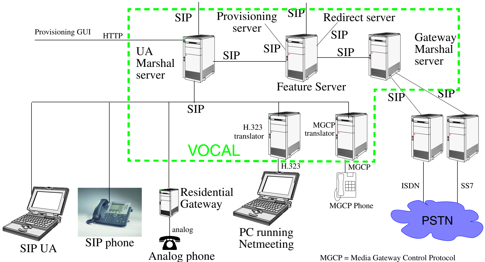
Figure 20: VOCAL: Simplified overview
