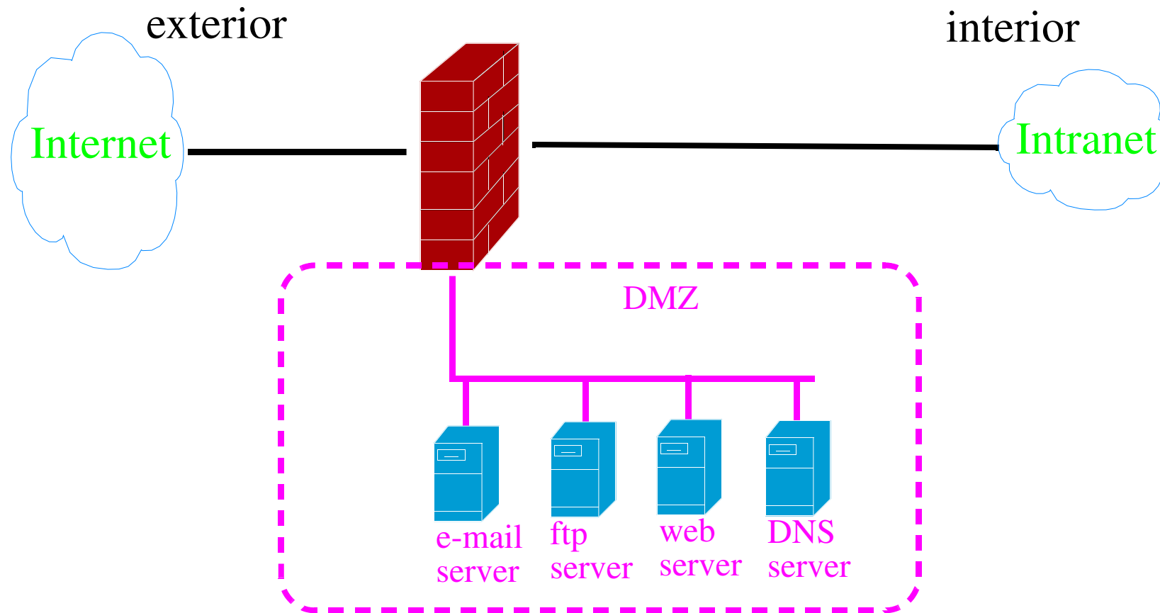
Figure 10: Example of a Firewall with a DMZ
