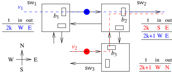
Fig. 1. Open-ended virtual circuits
