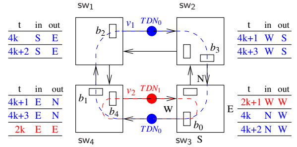
Fig. 2. Closed-loop virtual circuits
