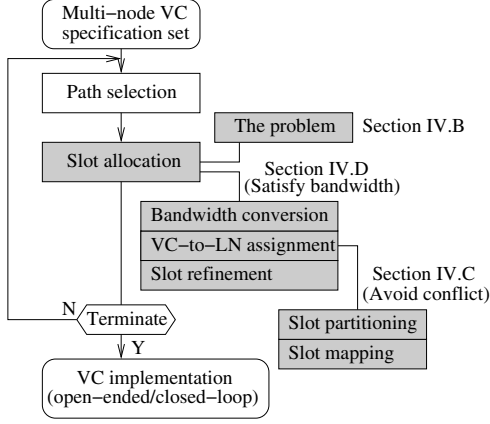
Fig. 3. Slot allocation in a VC configuration flow
