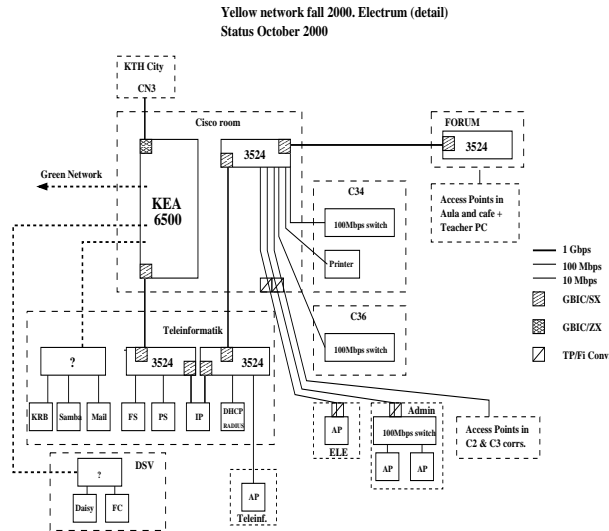
Figure 1: Yellow network topology at IT-University
