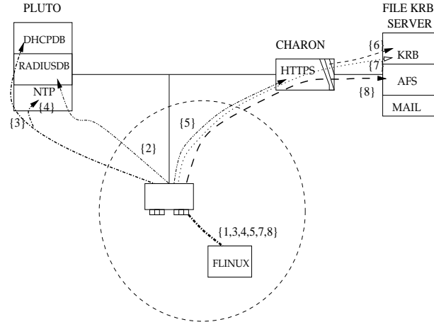
Figure 2: Authentication and wireless access in the IT-University Yellow network. Providing security in 802.11b.
