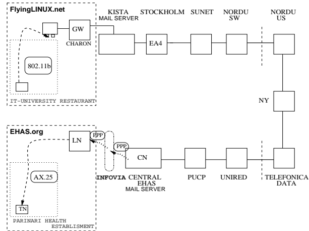
Figure 3: Wireless bits from the the restaurant at the new IT-University in Kista (Sweden) reaching an isolated health establishment in Parinari in the Peruvian Amazonia.
