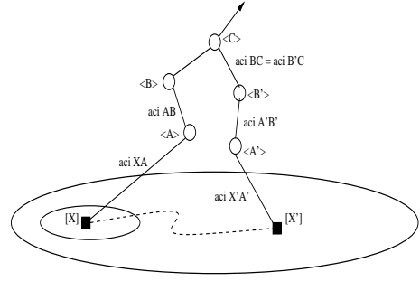
Figure 2: Case 0: ROUTE CREATE AIP_{exit} = AIP_{switch}
