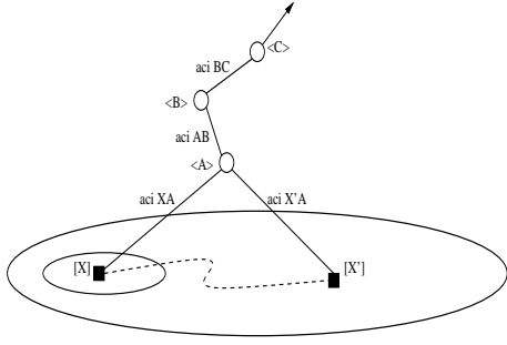
Figure 3: Case 1: ROUTE CREATE AIP_{entry} = AIP_{switch}
