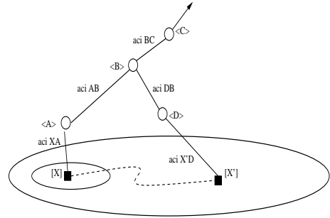
Figure 4: Case 2: ROUTE CREATE AIP_i = AIP_{switch}
