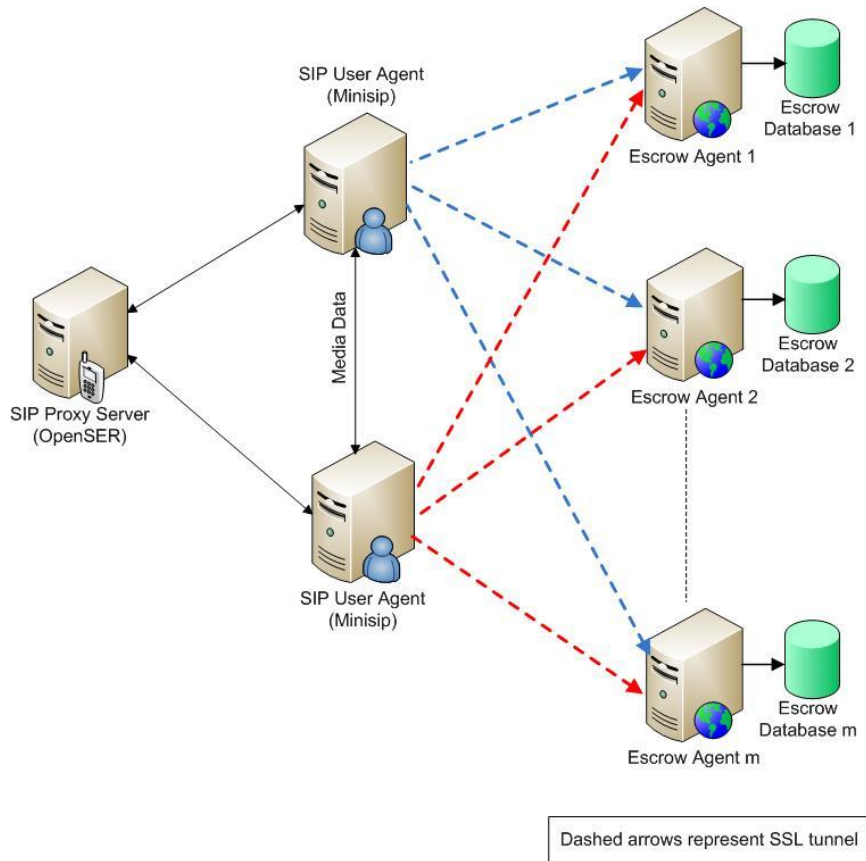
Figure 4-1: General architecture of m Escrow agents
