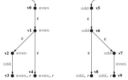
Figure 2: Flow graph of EvenOdd
